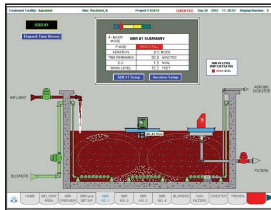
A typical SCADA system AquaSBR® basin detail screen depicting equipment status
