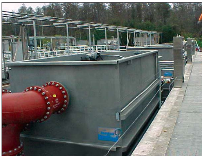
Orange County's North Plant AquaDisk® Filters.
